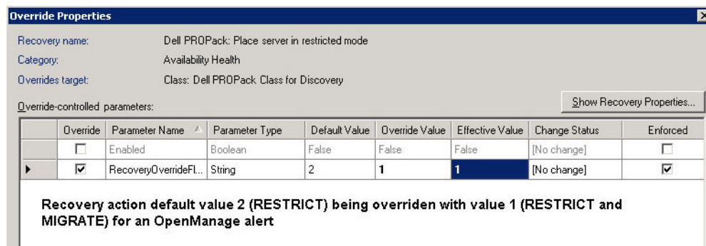
Figure 2. Override Properties
